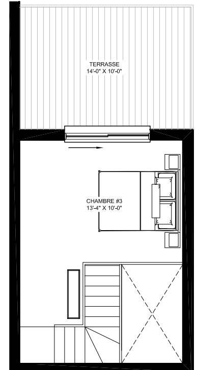
MEZZANINE
